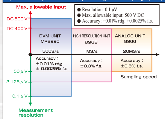
Input Unit Comparison Chart (Input Voltage and Sampling Speed)
