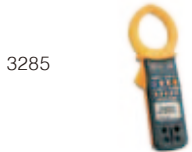
With the Memory HiCorder connection requires Output Cord 9094 and Conversion Adapter 9199
