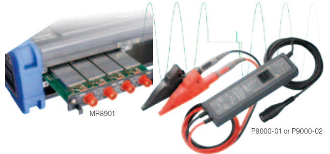
NEW The Differential Probe P9000 can be used with the standard Analog Unit MR8901 to enable high-voltage, 1,000 V (CAT III) measurement. The P9000-02 further enables RMS level measurement of AC power lines.
